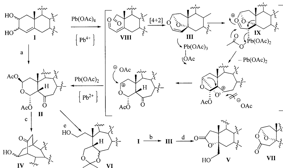
Scheme 1. Reagents and conditions: (a) 2.4 equiv. \text{Pb}(\text{OAc})_4 , MeCN, 0 °C to room temp.; (b) 1.2 equiv. \text{Pb}(\text{OAc})_4 , MeCN, 0 °C to room temp.; (c) \text{K}_2\text{CO}_3/\text{MeOH}/\text{H}_2\text{O} , room temp.; (d) \text{O}_3 , \text{CH}_2\text{Cl}_2 at -78 °C, then \text{K}_2\text{CO}_3/\text{MeOH}/\text{H}_2\text{O} , room temp.; (e) \text{LiAlH}_4 , THF, reflux then \text{H}^+ -acetone room temp.
