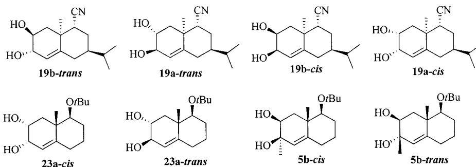
Scheme 5. Some of the diastereomerically pure unsaturated 1,2-diols examined
