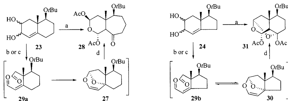
Scheme 8. Reagents and conditions: (a) 2.4 equiv. of \text{Pb}(\text{OAc})_4 in dry MeCN, -20^\circ\text{C} to room temp.; (b) 1.2 equiv. of \text{PhI}(\text{OAc})_2 in acetonitrile, 15–24 h at room temp.; (c) 4 equiv. of \text{Mn}(\text{OAc})_3 in refluxing MeCN; (d) 1.2 equiv. of \text{Pb}(\text{OAc})_4 in dry MeCN at room temp.
