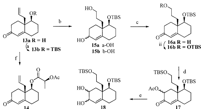
Scheme 3. Reagents and conditions: (a) \text{TBSCl} , \text{DMF}/\text{imidazole} , 0^{\circ}\text{C} , 24 h (89%). (b) \text{BH}_3 \cdot \text{Me}_2\text{S} , \text{H}_2\text{O}_2/\text{NaOH} , \text{EtOH} , 8 h (78%). (c) i. \text{PCC} , 3,5- \text{DMP} , 0^{\circ}\text{C} (62%); ii. \text{TBSCl} , \text{DMF}/\text{imidazole} , 0^{\circ}\text{C} , 1.5 h (91%); (d) \text{Pb}(\text{OAc})_4 , \text{PhH} , reflux, 4 d (90%); (e) \text{LiAlH}_4/\text{Et}_2\text{O} , 0^{\circ}\text{C} , 30 min (99%); (f) ( S )-2-acetoxypentenyl chloride, \text{DMAP} , \text{CH}_2\text{Cl}_2 , 0^{\circ}\text{C} , 30 min.
