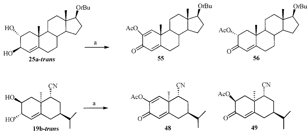
Scheme 6. Reagents and conditions: (a) Dess–Martin periodinane (2 equiv.), dry PhMe, room temp. to 72 °C, ca. 1 h, then cool to 0 °C, Ac 2 O/py, DMAP
