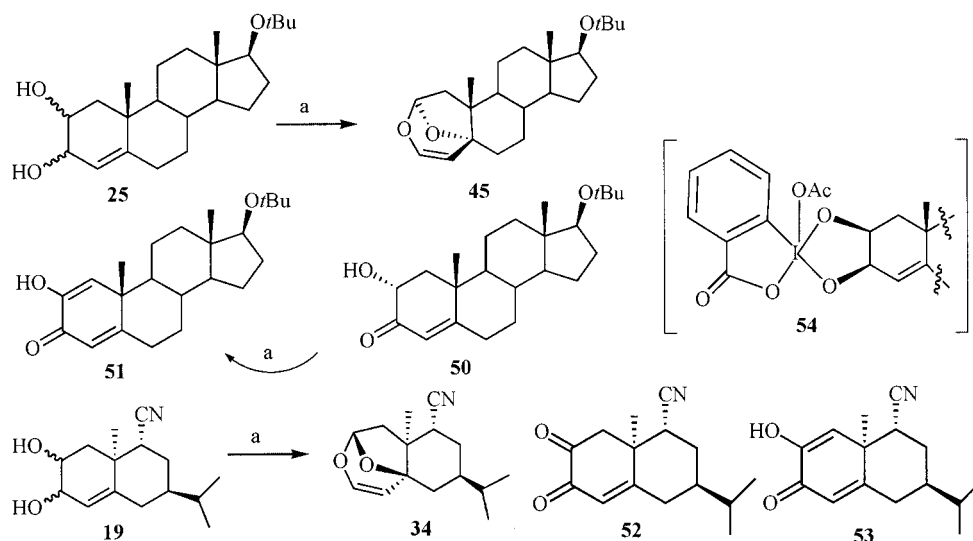
Scheme 4. Reagents and conditions: (a) 2 equiv. Dess–Martin periodinane in dry PhMe, room temp. to 72 °C
