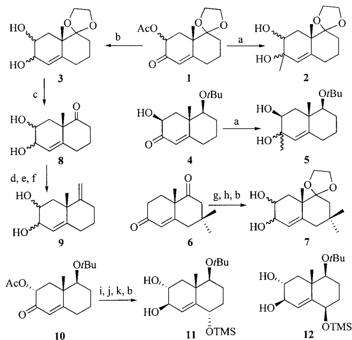
Scheme 2. Reagents and conditions: (a) MeLi, THF, -78^{\circ}\text{C} (86–90%); (b) \text{LiAlH}_4/\text{Et}_2\text{O} , 0^{\circ}\text{C} (99%); (c) 10% \text{HCl}/\text{THF} , 1:1, 4^{\circ}\text{C} , 12 h (99%); (d) \text{TBSCl} , \text{DMF}/\text{imidazole} , 0^{\circ}\text{C} , 2 h (87%); (e) \text{PPh}_3\text{MeBr} , t\text{BuOK} , \text{PhMe} , room temp., 4 h (94%); (f) \text{TBAF}/\text{THF} , 60^{\circ}\text{C} , 4 h (96%); (g) ethylene glycol, p\text{-TosH} , room temp. (95%); (h) 4 equiv. \text{Pb}(\text{OAc})_4 , benzene, 90^{\circ}\text{C} , 4 d (85%); (i) \text{Ac}_2\text{O} , \text{Py} , 4- \text{DMAP} , 80\text{--}100^{\circ}\text{C} (90%); (j) \text{MTO} , 30% \text{H}_2\text{O}_2 , \text{Py} , \text{CH}_2\text{Cl}_2 , room temp. (70%); (k) \text{TMSOTf} , collidine, \text{PhMe} , -40^{\circ}\text{C} (95%)
