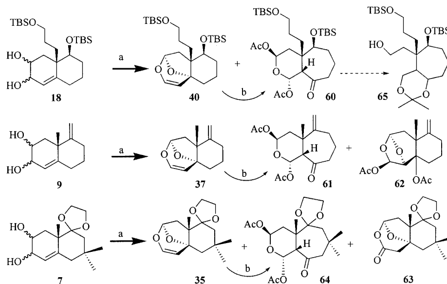
Scheme 9. Reagents and conditions: (a) 2.4 equiv. \text{Pb}(\text{OAc})_4 , \text{AcOH} , room temp., 17 h; (b) 1.2 equiv. \text{Pb}(\text{OAc})_4 , \text{AcOH} , room temp., 17 h
