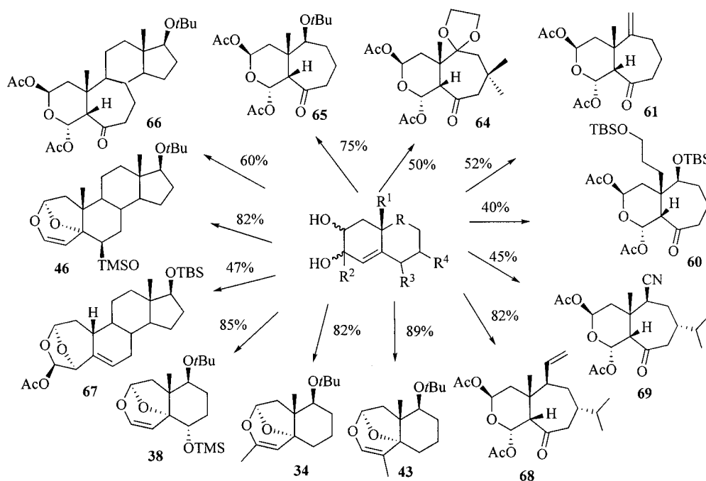
Scheme 10. Reagents and conditions: 2.4 equiv. \text{Pb}(\text{OAc})_4 in \text{AcOH} at room temp.
